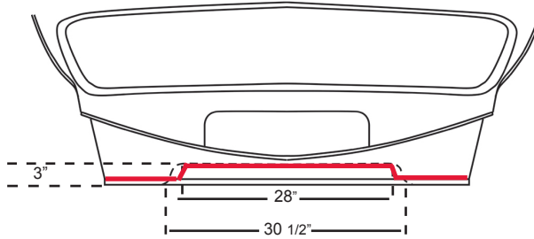
481000 48-52 TRUCK FIREWALL
